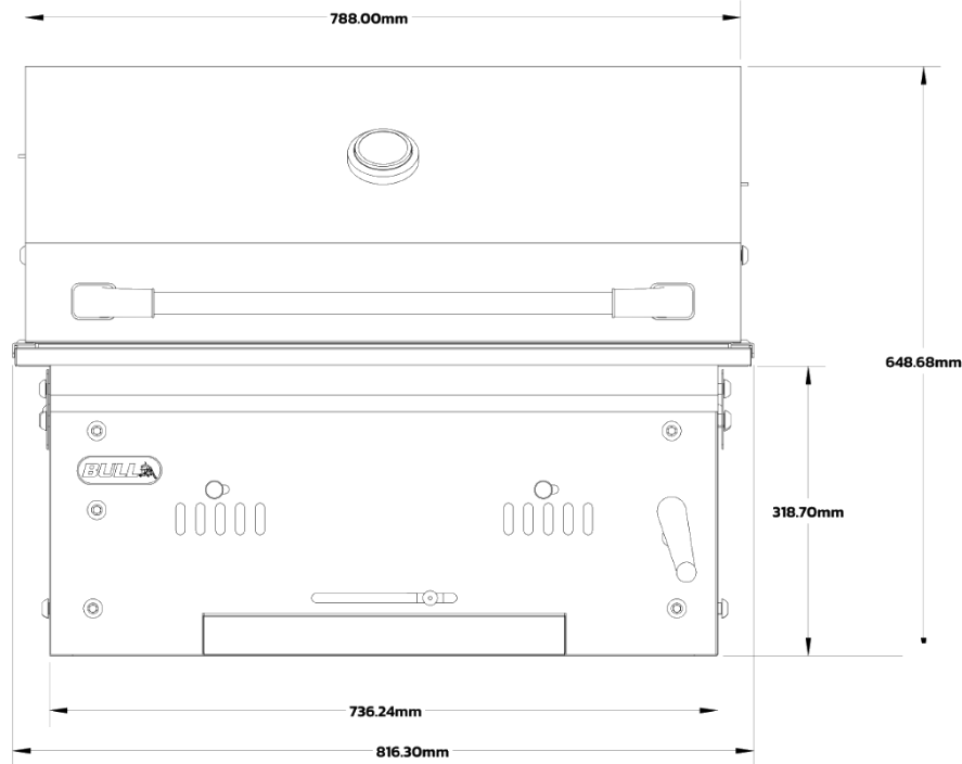
FRONT VIEW 816.30 W × 648.68 H mm
