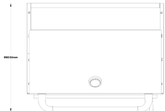
TOP VIEW 736.24 W × 650.52 D mm
