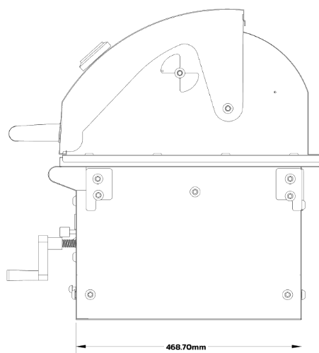
SIDE VIEW 468.70 D × 318.70 H mm
